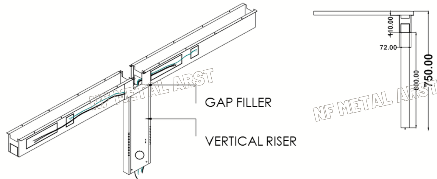
C SHAPE RACEWAY-ACCESS FROM BELOW TOP NON SHARING (ONE SIDE CUTOUT)
