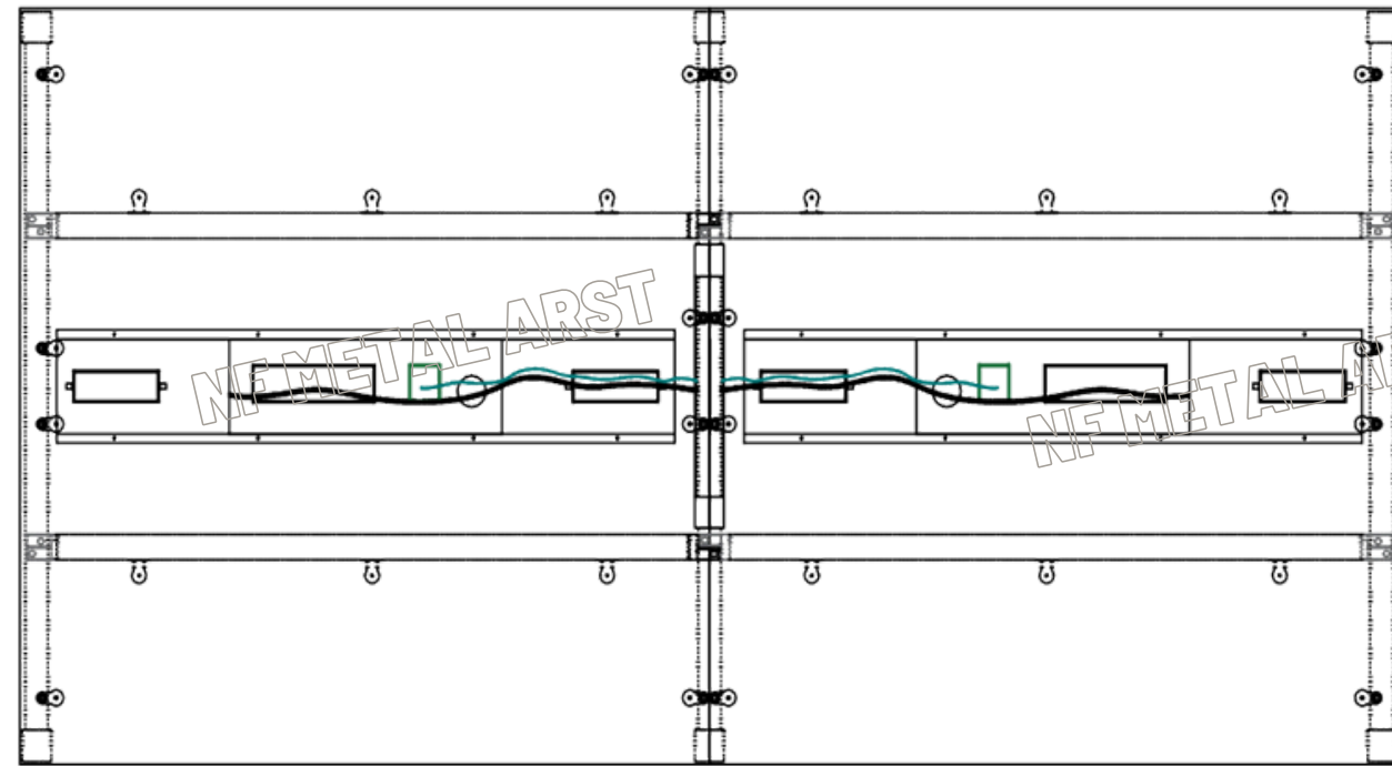
C SHAPE RACEWAY FOR CONFERENCE/MEETING TABLE - ACCESS FROM ABOVE TOP
