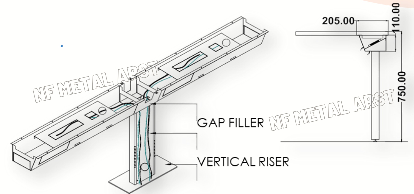
C SHAPE RACEWAY-ACCESS FROM ABOVE TOP NON SHARING (ONE SIDE CUTOUT)
