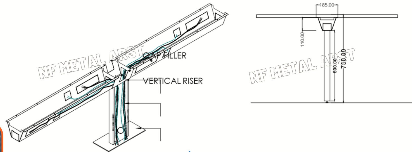
C SHAPE RACEWAY-ACCESS FROM BELOW TOP SHARING (BOTH SIDE CUTOUT)
